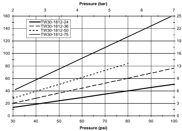
Figure 2. Impact of Pressure on Permeate Flow (constant temperature, recovery)
